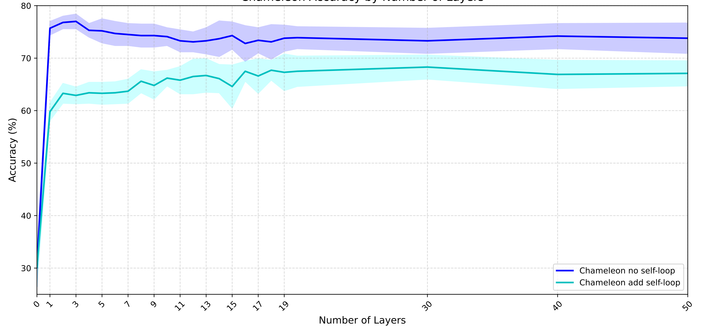
Chameleon Accuracy by Number of Layers
